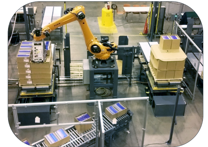
Robot placing cases on a pallet
