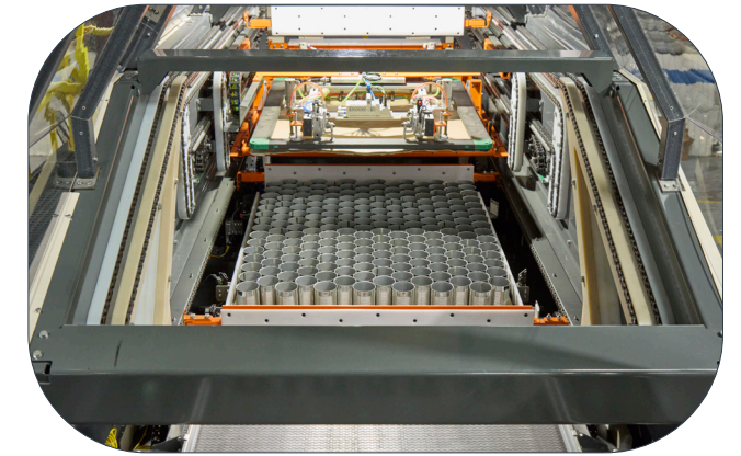
Sweeping a layer of cans onto accumulator
