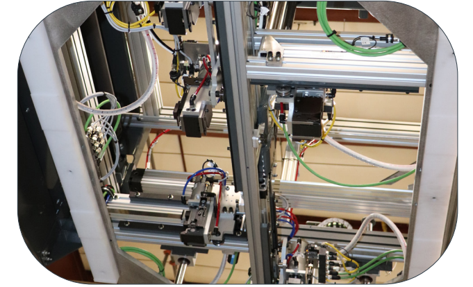
Destrapper cutting head assembly
